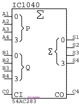
54AC283 IC????
