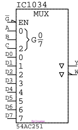
54AC251 IC????
