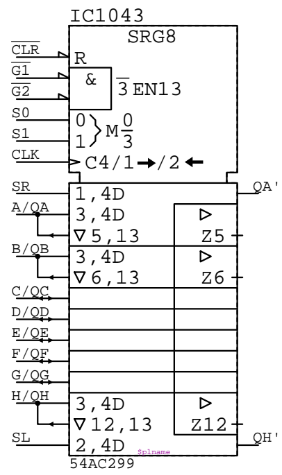
54AC299 IC????
