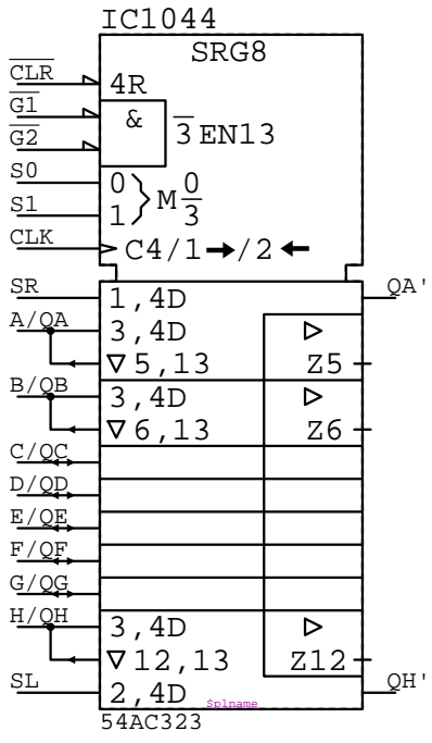
54AC323 IC????
