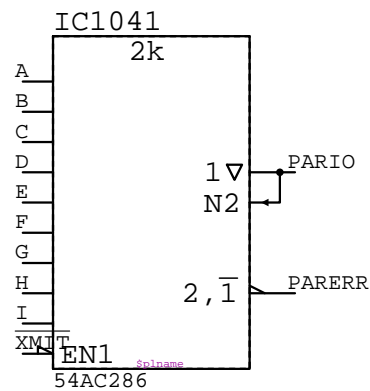
54AC286 IC????
