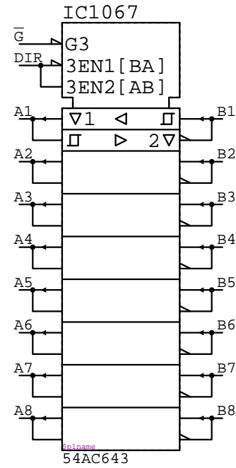
54AC643
