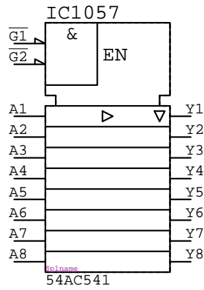
54AC541 IC?????
