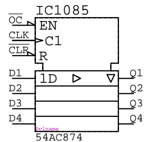
54AC874 IC????
