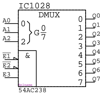
54AC238 IC????
