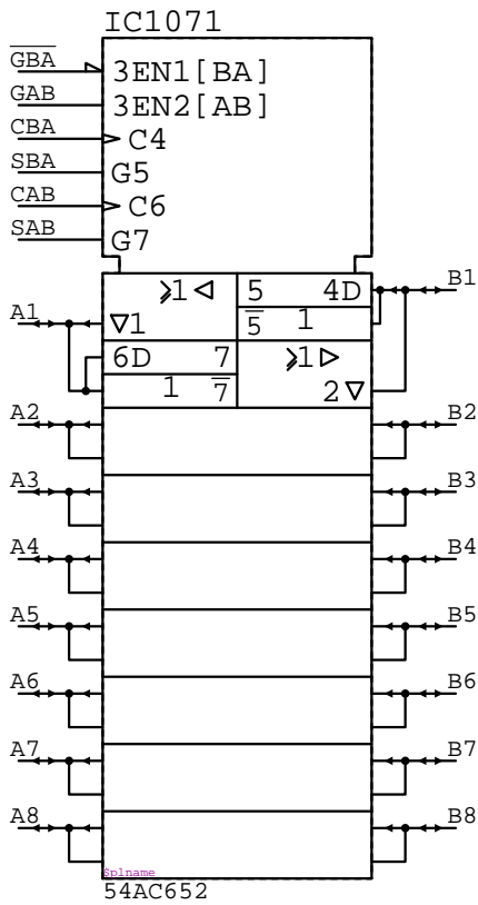
54AC652 IC?????
