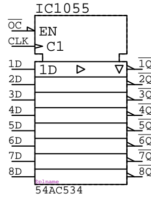
54AC534 IC?????
