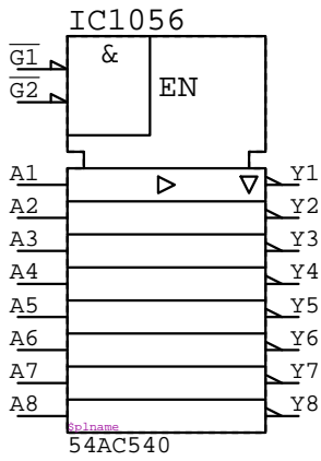
54AC540 IC?????
