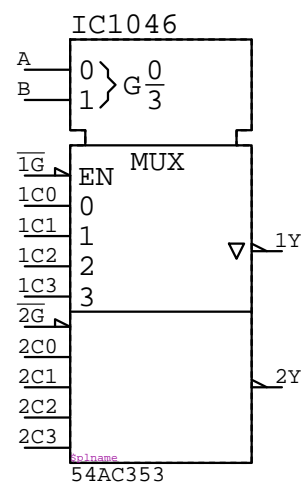
54AC353 IC????
