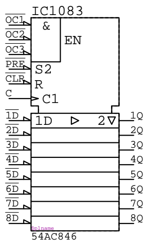
54AC846 IC????
