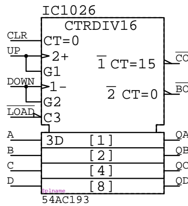
54AC193 IC????
