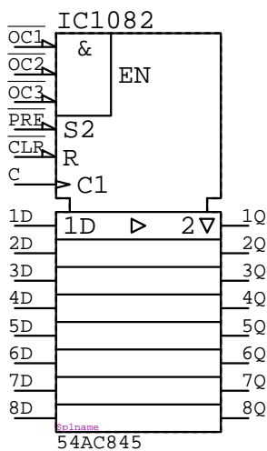
54AC845 IC????
