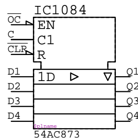
54AC873 IC????
