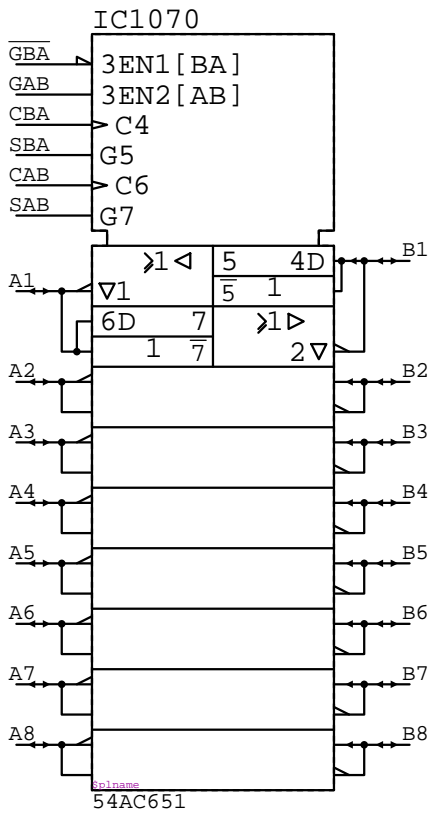
54AC651 IC?????
