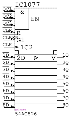
54AC826 IC????
