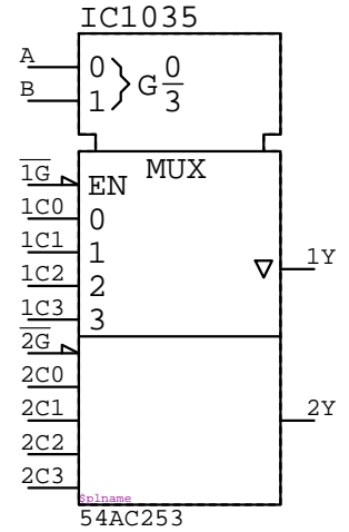
54AC253 IC????
