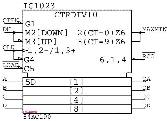
54AC190 IC????
