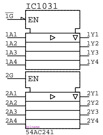
54AC241 IC????
