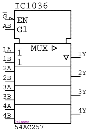
54AC257 IC????
