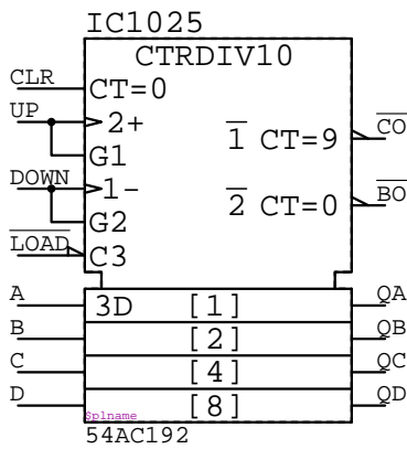
54AC192 IC????
