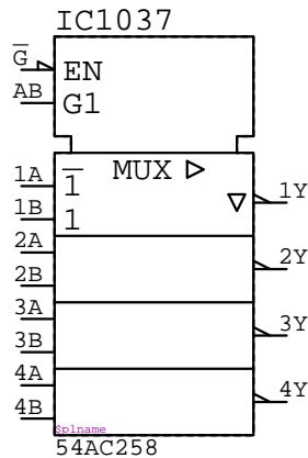
54AC258 IC????
