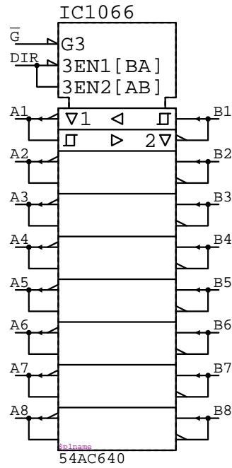
54AC640
