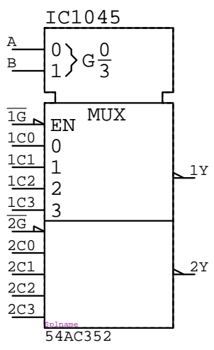
54AC352 IC????
