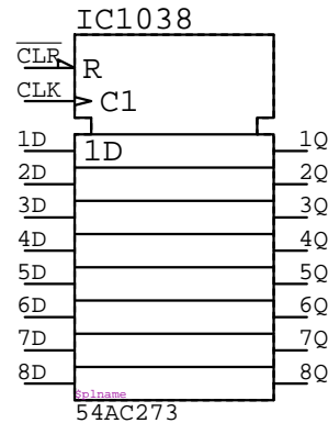
54AC273 IC????
