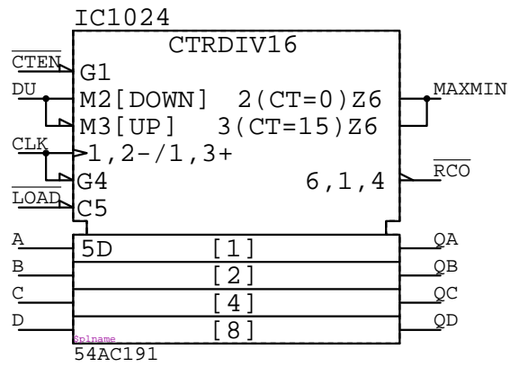
54AC191 IC????
