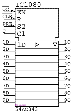
54AC843 IC????
