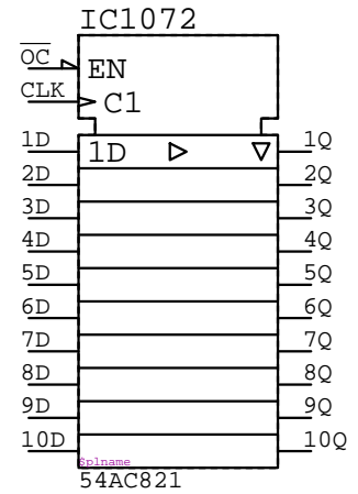
54AC821 IC?????
