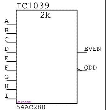
54AC280 IC????
