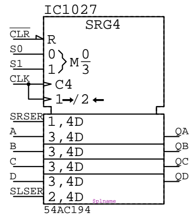
54AC194 IC????
