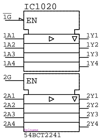
54BCT2241
