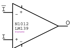
OP_LM139 N????
