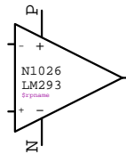
OP_LM293SUPPLY N????
